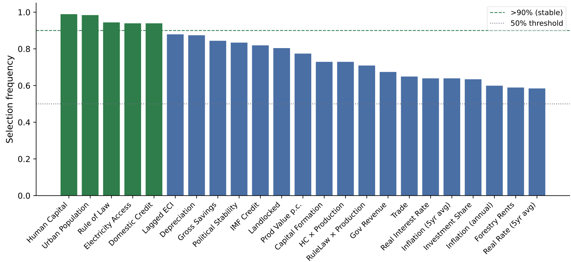
LASSO Selection Frequency Across Bootstrap Samples (B = 200)
